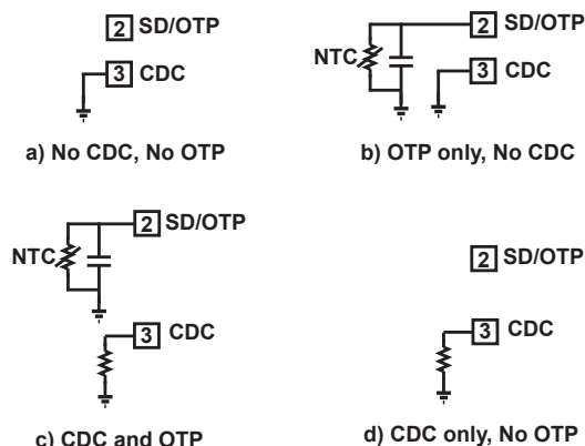
Figure 9.5: CDC and SD/OTP Pins Configurations
