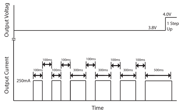
Figure 9.6: Increase Output Voltage Command
