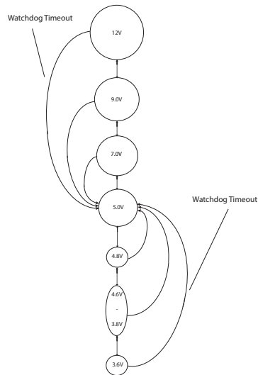
Figure 9.8: State Machine
