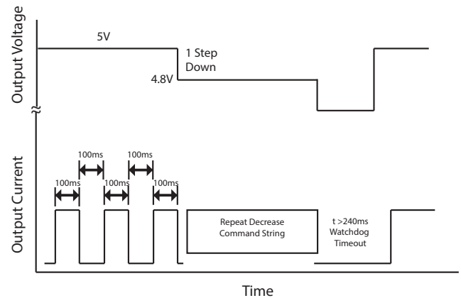
Figure 9.9: Watchdog Timeout
