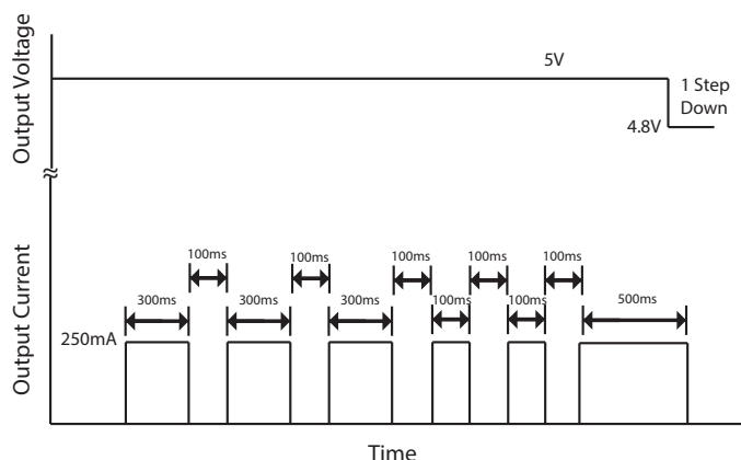
Figure 9.7: Command to Decrease Output Voltage
