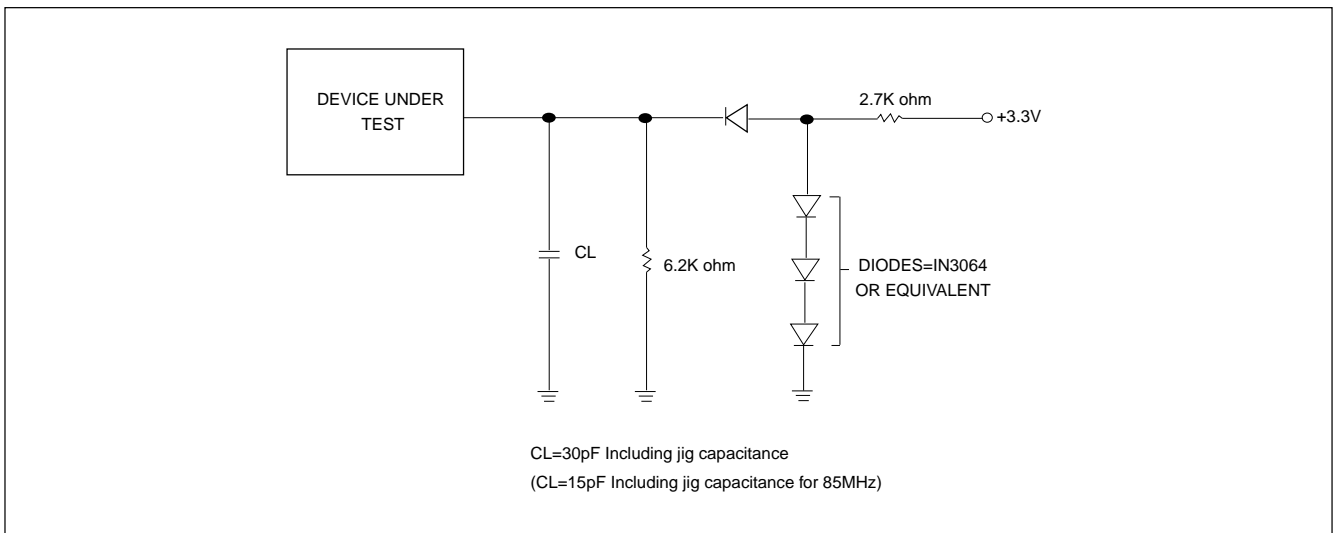
Figure 6. OUTPUT LOADING
