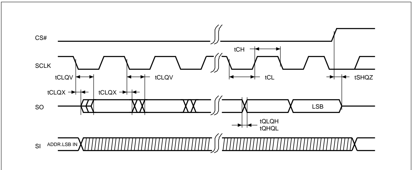
Figure 8. Output Timing
