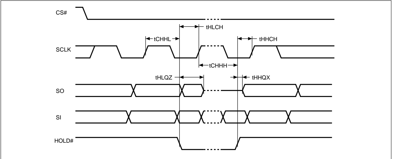
Figure 9. Hold Timing
