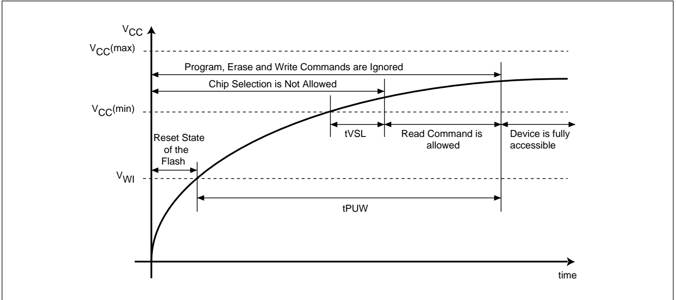
Figure 26. Power-up Timing
