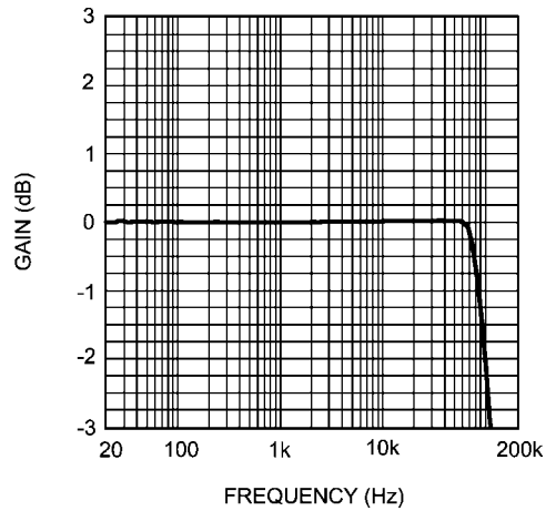
Closed Loop Frequency Response +V_{CC} = -V_{EE} = 50V, V_{IN} = 1V_{RMS}
