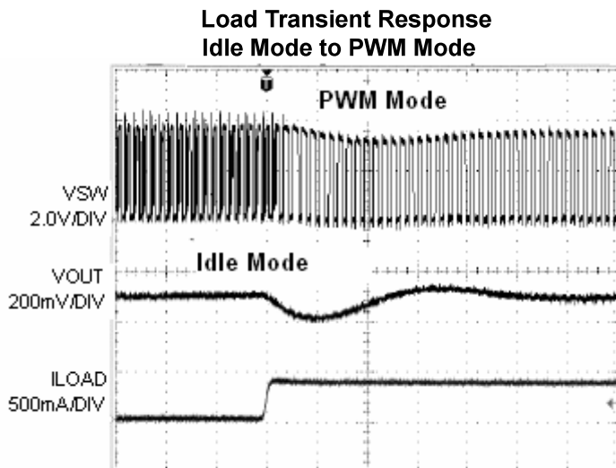
I_{load}=28mA to 400mA , L=2.2\mu H , C_{in}=10\mu F , C_{out}=10\mu F , V_{in}=3.6V , V_{out}=1.8V
