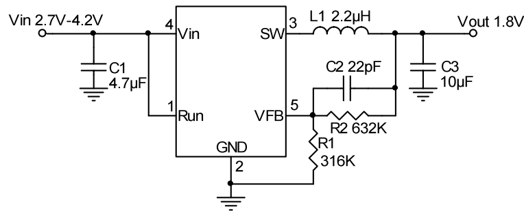
Fig.1 Basic Application Circuit with AM2406 adjustable version
