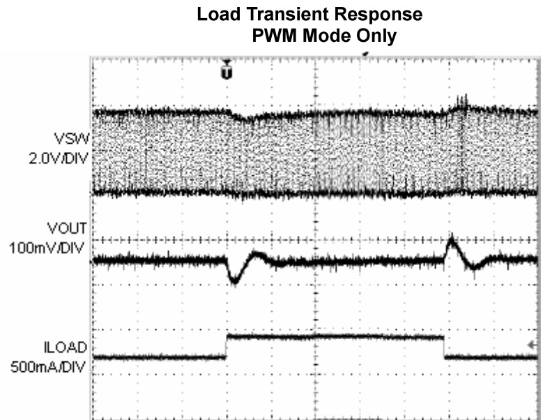
I_{LOAD}=100mA to 400mA L=2.2\mu H , C_{in}=10\mu F , C_{out}=10\mu F , V_{in}=3.6V , V_{out}=1.8V
