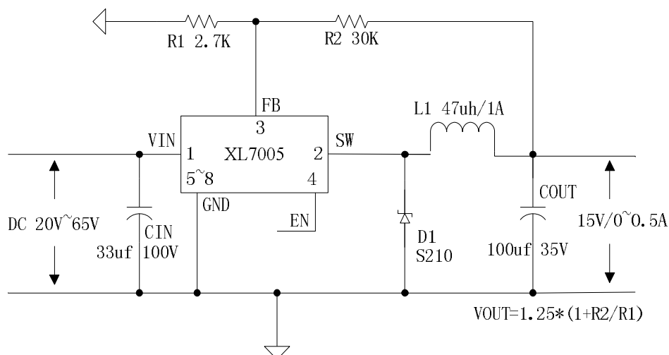
Figure5. XL7005 System Application ( V_{IN}=20V \sim 65V , V_{OUT}=15V )
