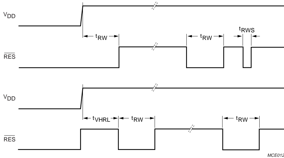
Fig.41 Reset timing.
