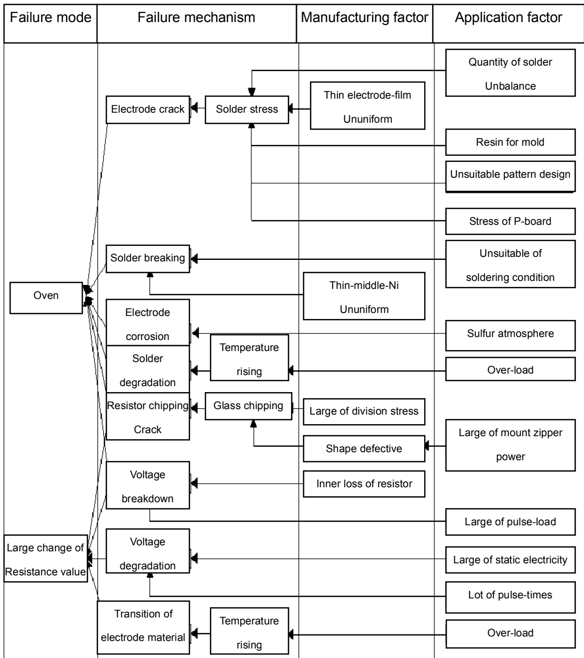
Fig.12. Failure mechanism
