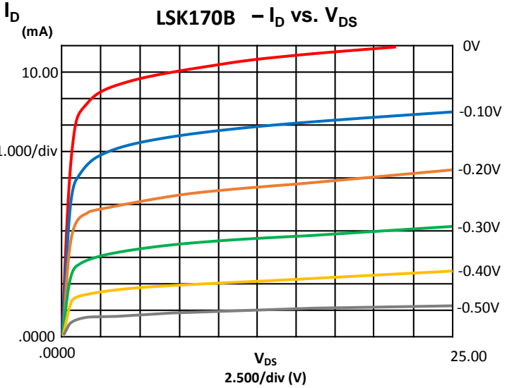
Output Characteristics
