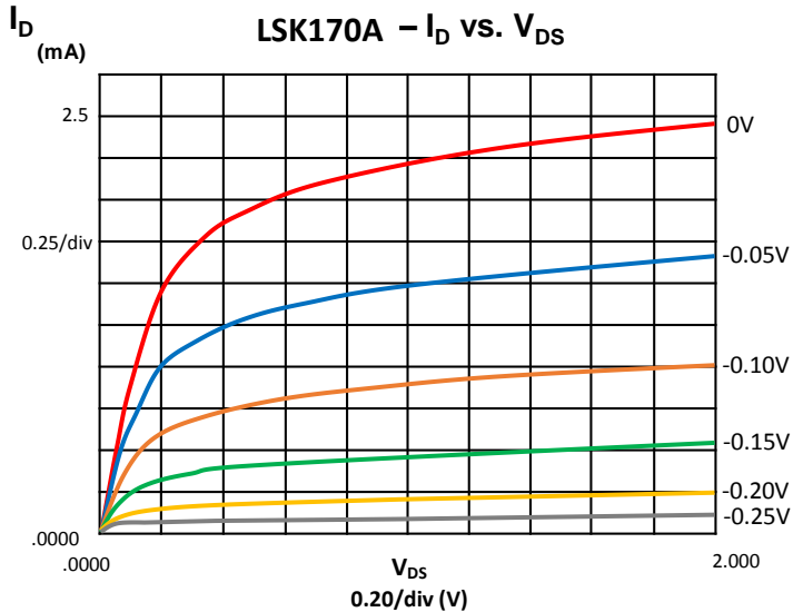
Operating Characteristics
