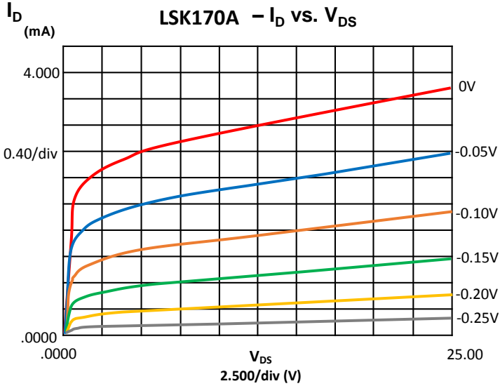
Output Characteristics
