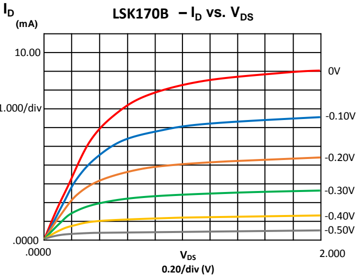
Operating Characteristics
