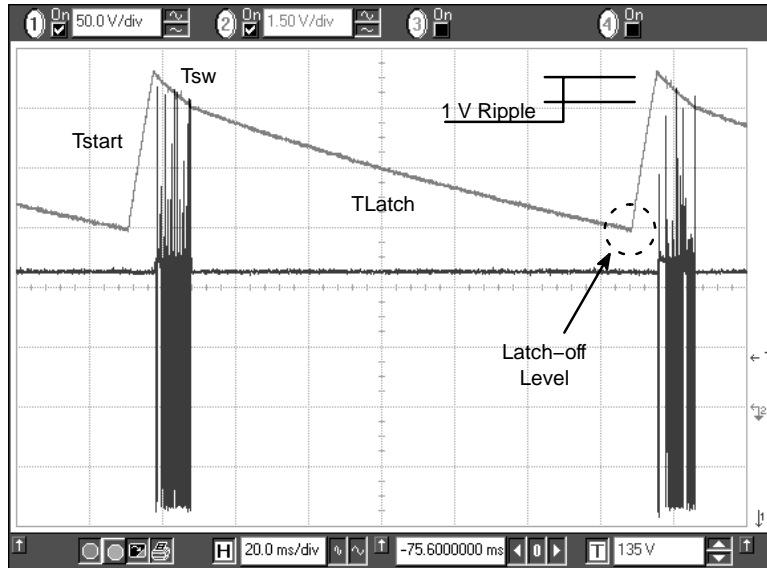
Figure 16. NCP101X Facing a Fault Condition (Vin = 150 Vdc)
