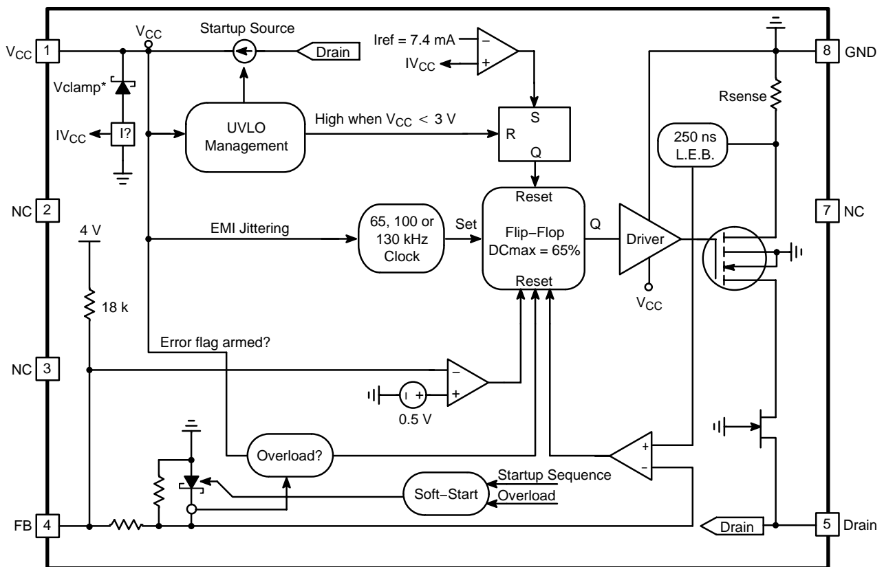
Figure 2. Simplified Internal Circuit Architecture
