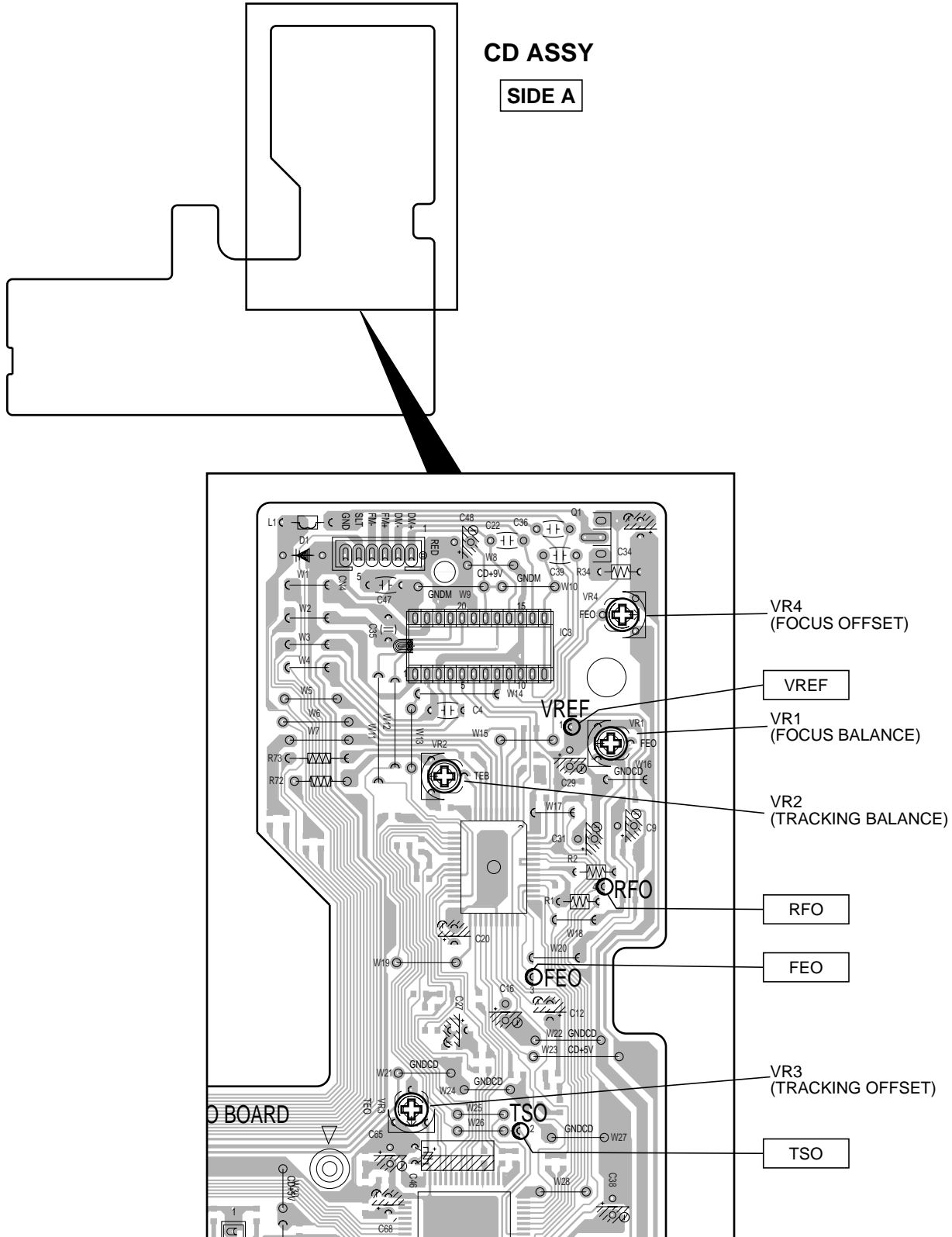
Fig. 1 Adjustment Locations
