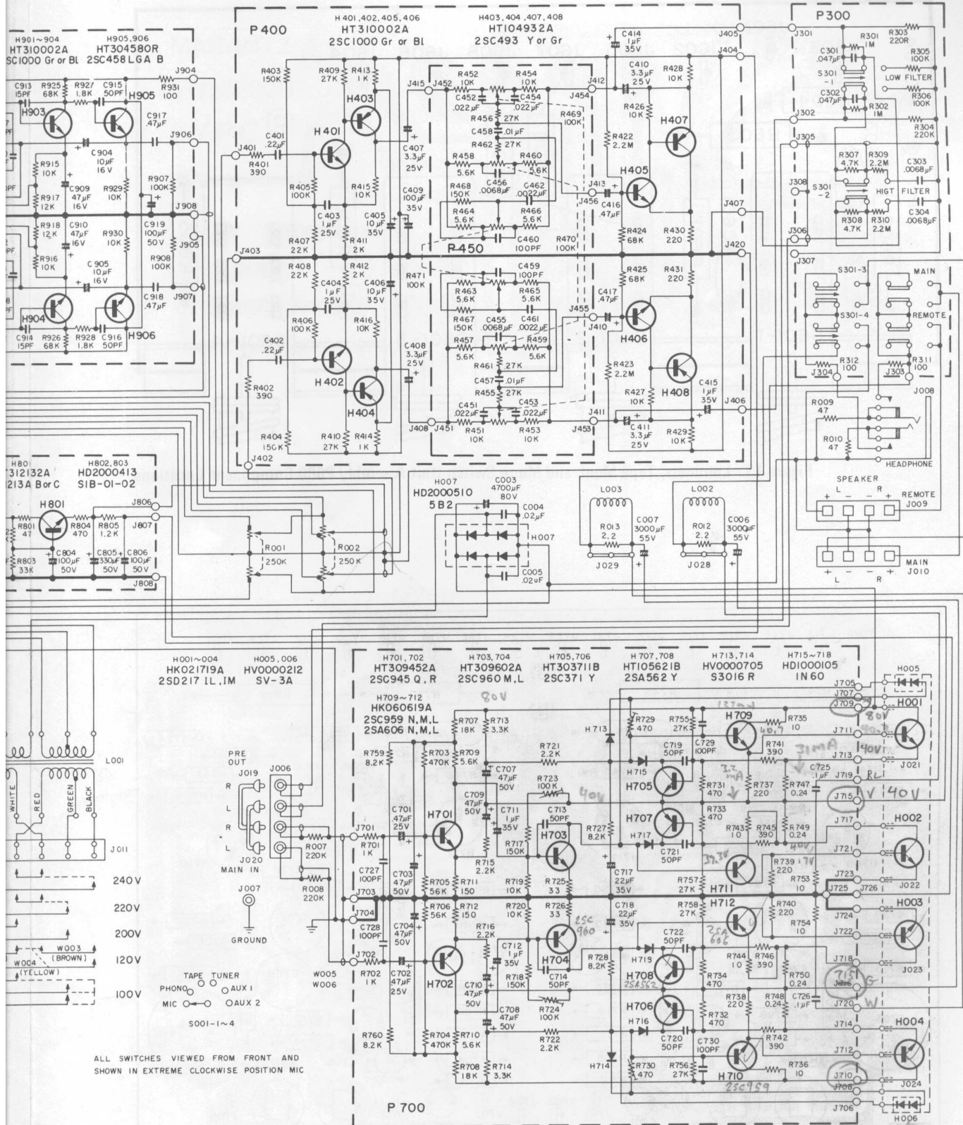
Figure 16. Schematic Diagram
