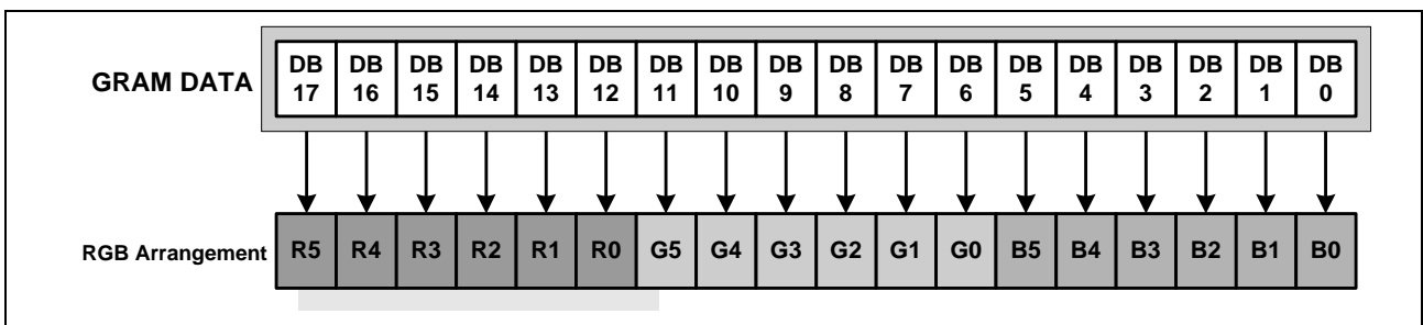
Figure 34. RAM Data Write Format for 80-system 18-bit Interface
