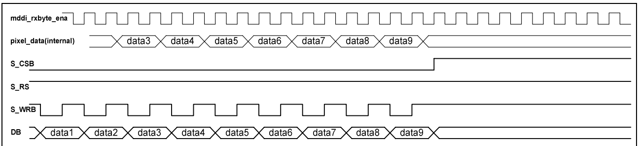
Figure 91. Change Data Path from Sub Panel to Main Panel
