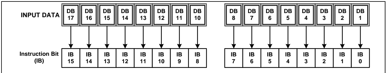
Figure 24. Instruction Format for 68-system 16-bit Interface
