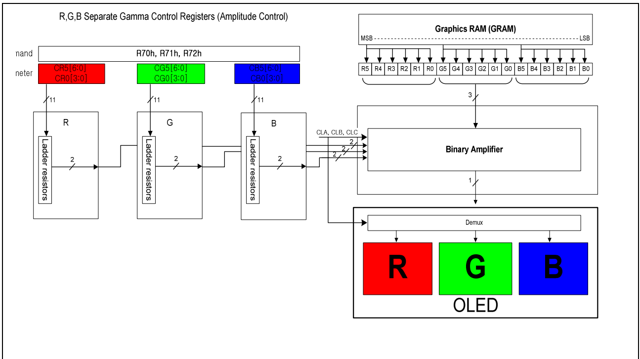
Figure 100. 8-color Display Control
