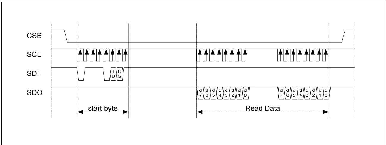
Figure 49. Timing Diagram of Register Read through SPI
