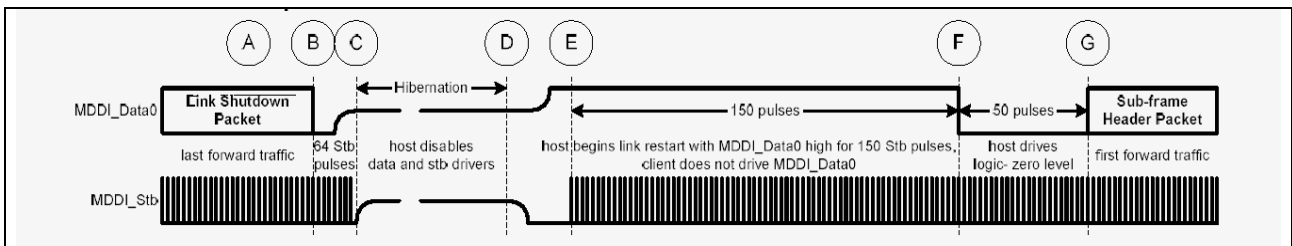
Figure 64. Host-initiated Link Wake-up Procedure
