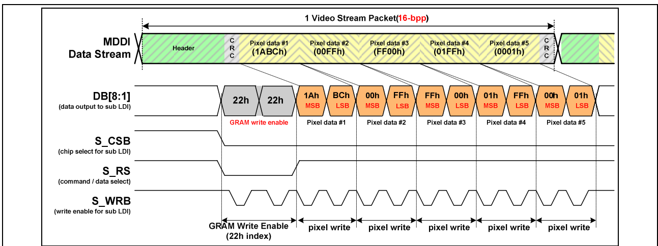
Figure 84. 80 Mode TFT Type 8-bit Video Data Transfer
