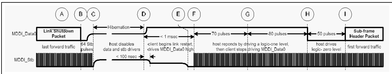
Figure 67. Client-initiated Link Wake-up Procedure
