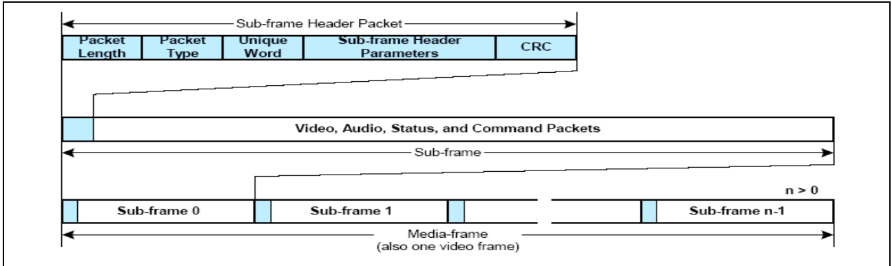
Figure 71. MDDI Packet Structure
