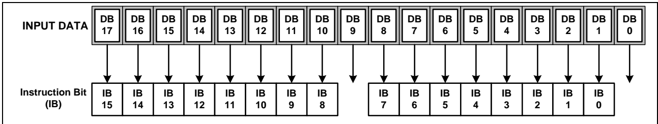
Figure 21. Instruction Format for 68-system 18-bit Interface
