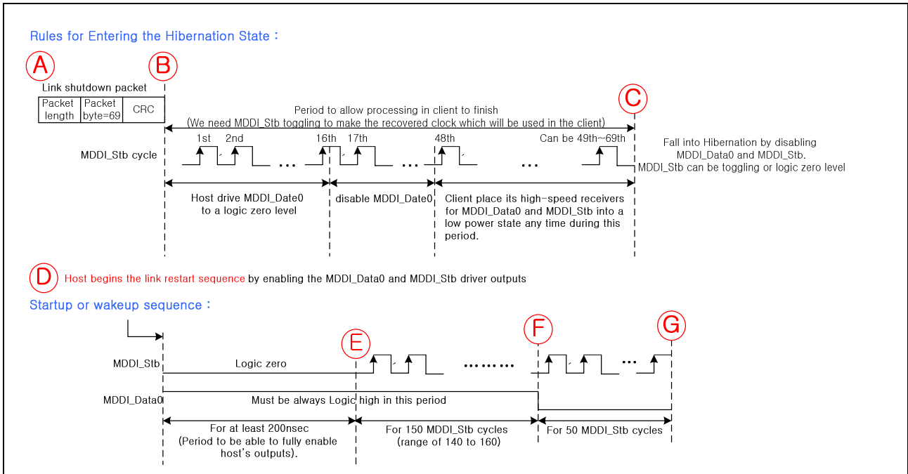
Figure 65. Host-initiated Link Wake-up Sequence
