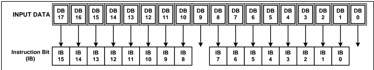
Figure 33. Instruction Format for 80-system 18-bit Interface
