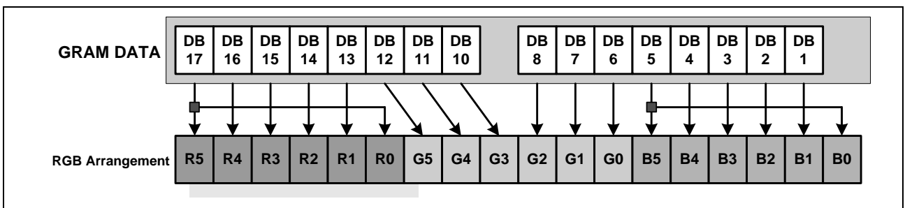
Figure 25. RAM Data Write Format for 68-system 16-bit Interface
