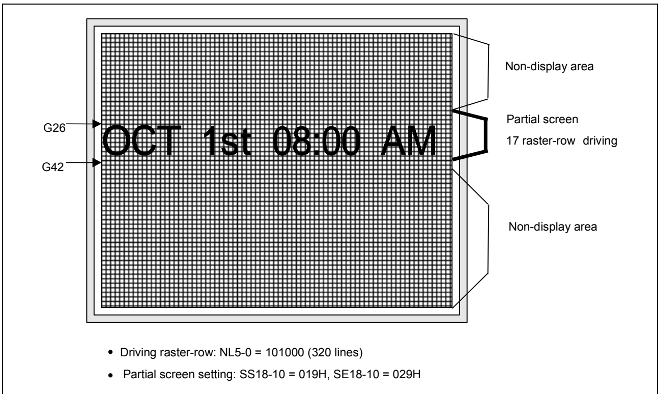
Figure 11. Driving On Partial Screen
