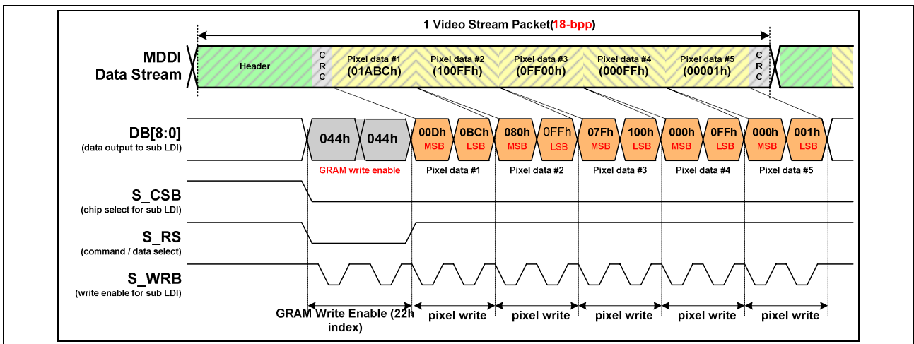
Figure 83. 80 Mode TFT Type 9-bit Video Data Transfer
