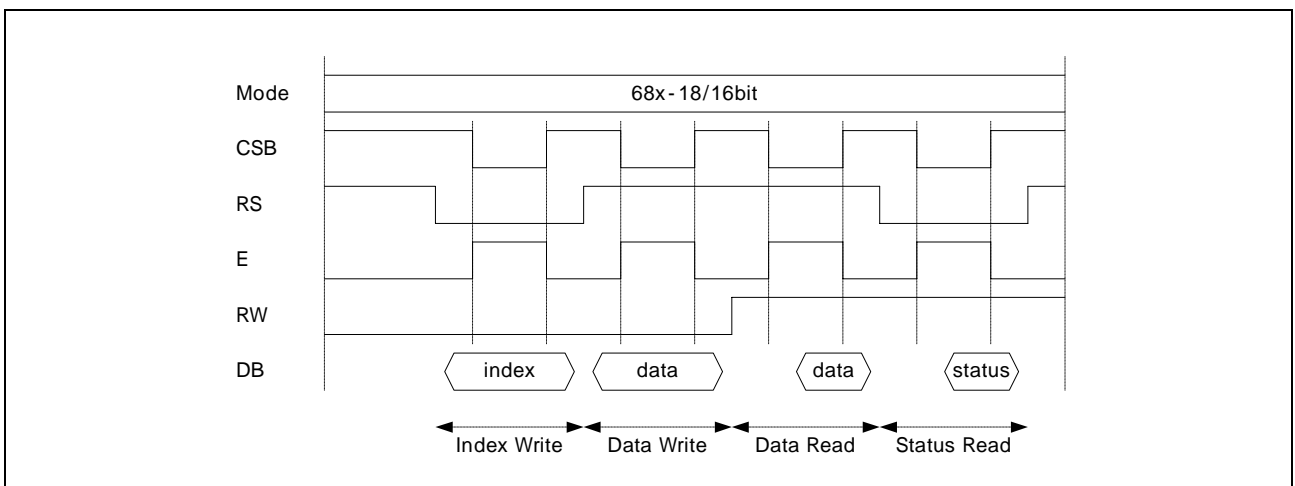
Figure 26. Timing Diagram of 68-system 16-bit Bus Interface
