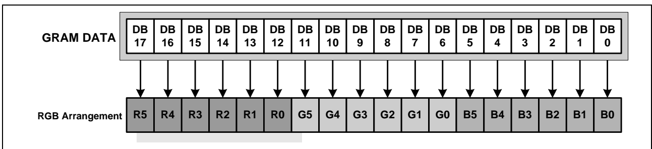
Figure 22. RAM Data Write Format for 68-system 18-bit Interface
