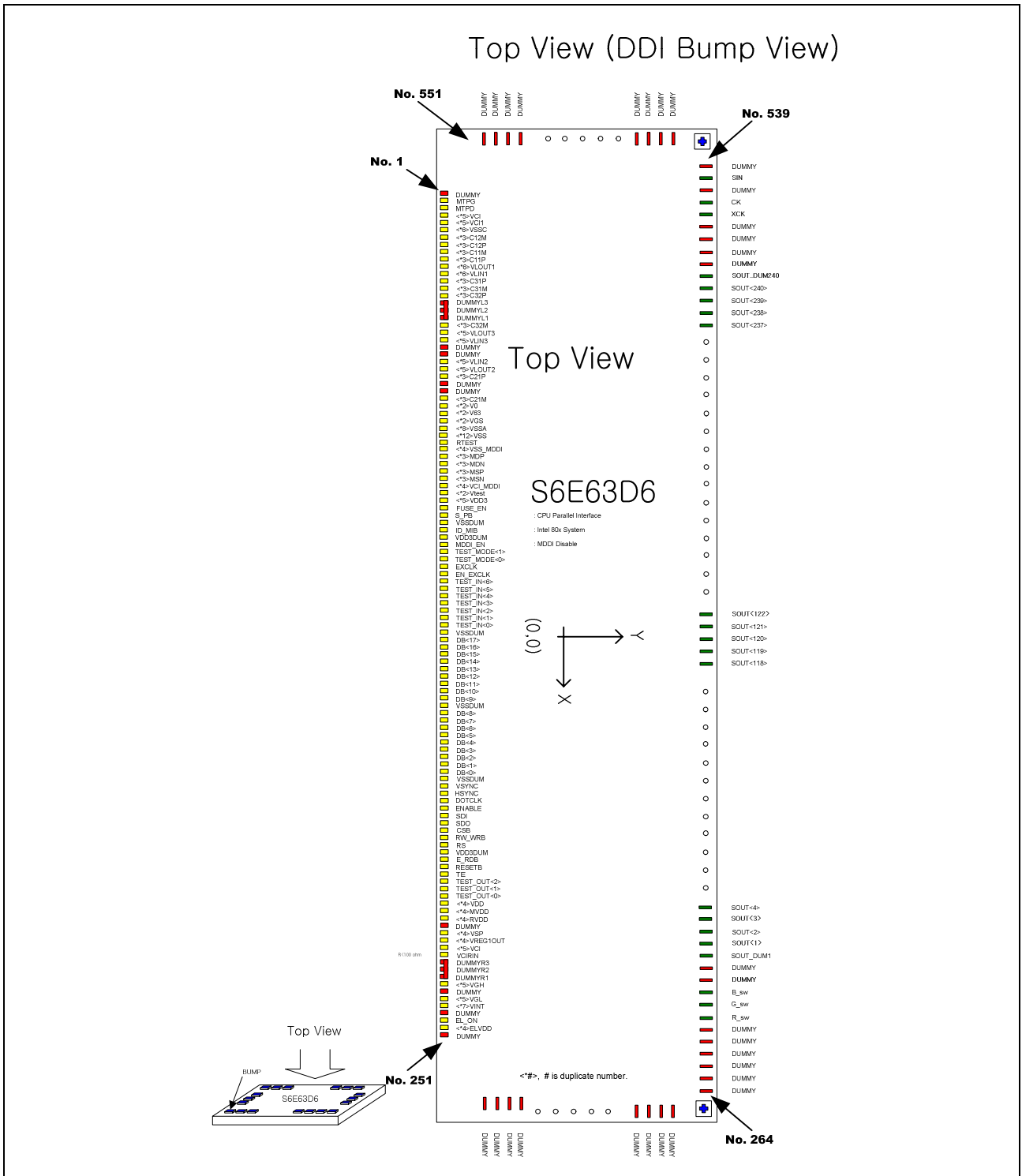
Figure 2. Pad Layout
