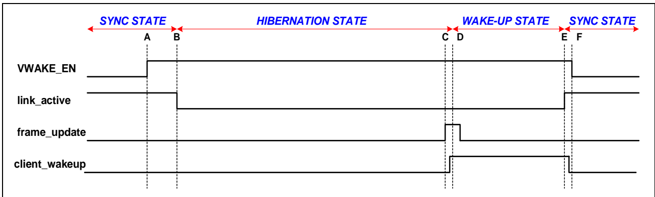
Figure 69. VSYNC Based Link Wake-up Procedure
