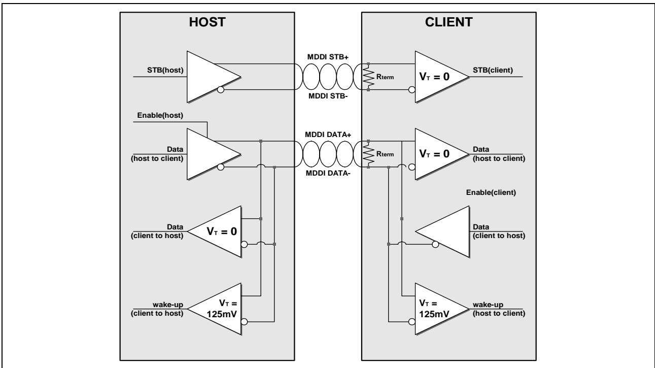
Figure 61. Differential Connection between Host and Client
