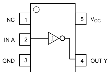
Figure 1. Pinout
