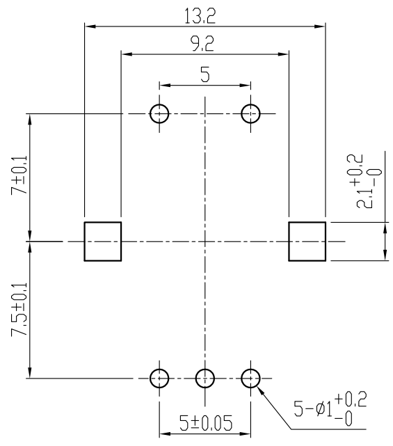
P.C.B.MOUNTING DETAIL
