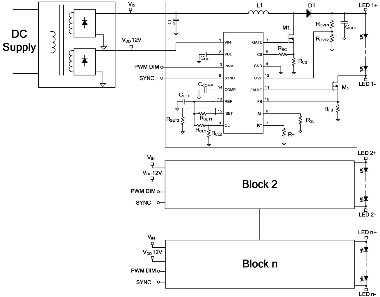
Figure 5—Typical Application Circuit for TV LED Backlighting
