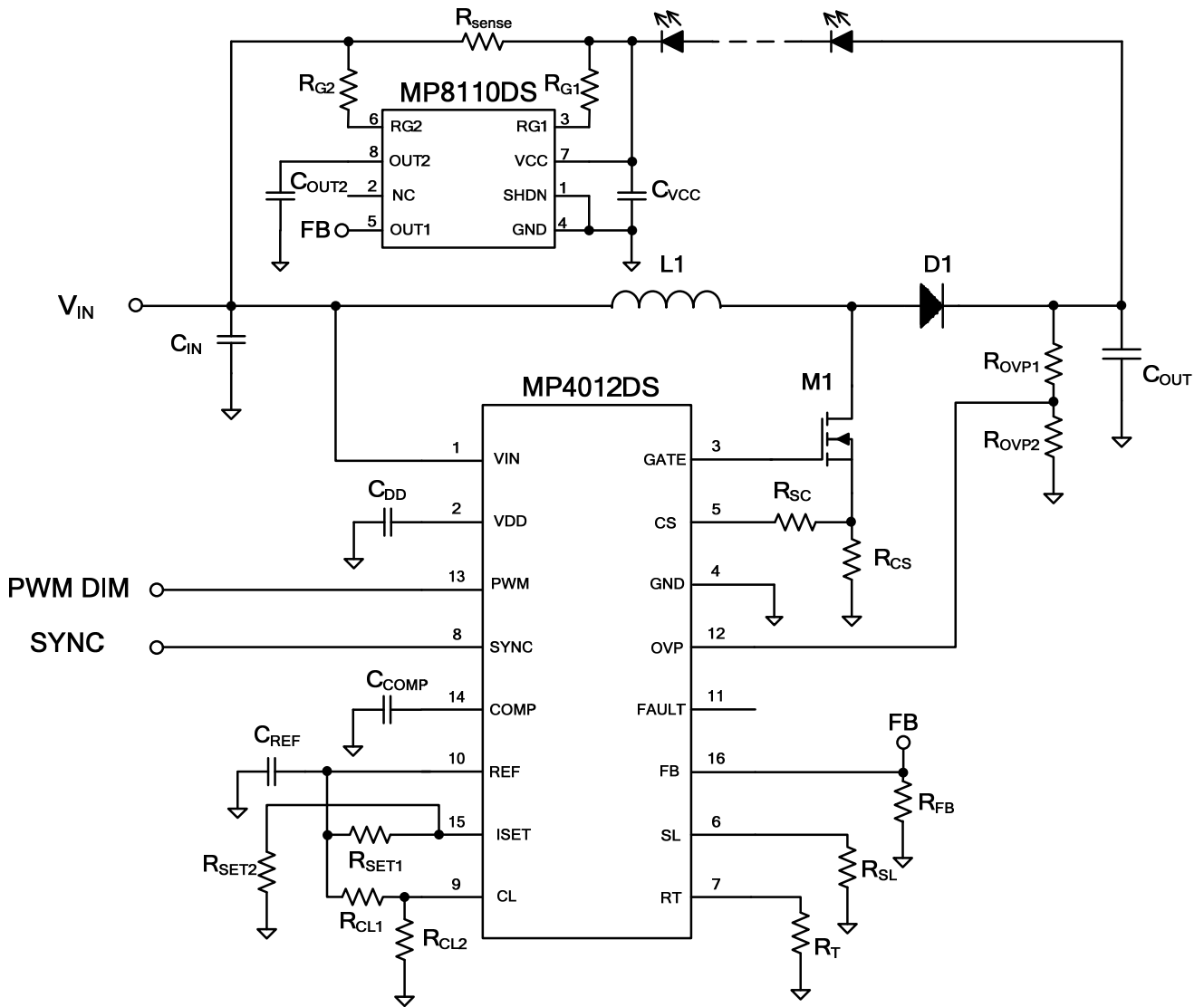
Figure 7—MP4012 Buck-Boost Application Circuit
