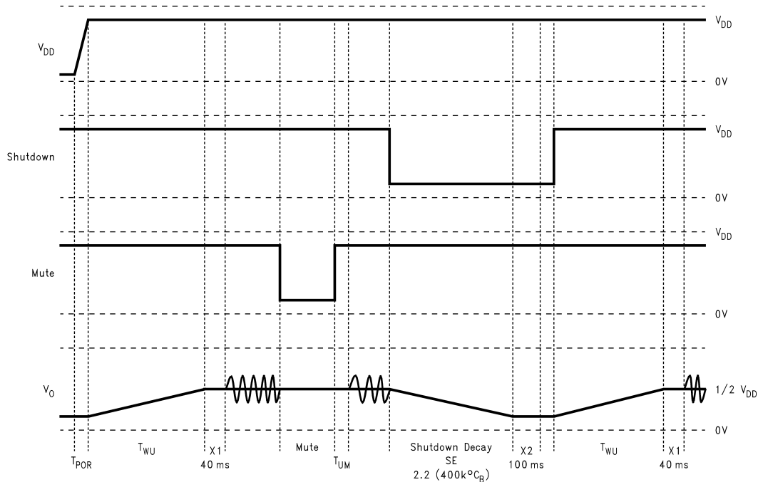
Figure 9. Turn-On, Shutdown, and Mute Timing for Cap-Coupled Mode
