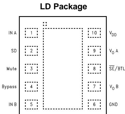
Figure 4. Top View Order Number LM4916LD See NS Package Number LDA10A
