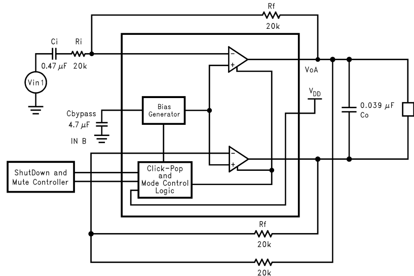
Figure 7. Typical BTL Speaker Configuration Circuit
