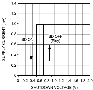
Shutdown Hysteresis Voltage V DD = 1.5V
