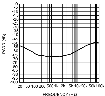
Power Supply Rejection Ratio V_{DD} = 1.2V , V_{RIPPLE} = 200mV_{PP} R_L = 8\Omega , BTL Input Terminated into 10\Omega
