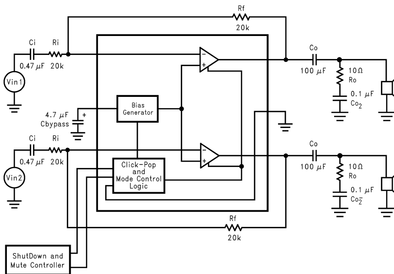
Figure 6. Typical Single Ended Output Configuration Circuit
