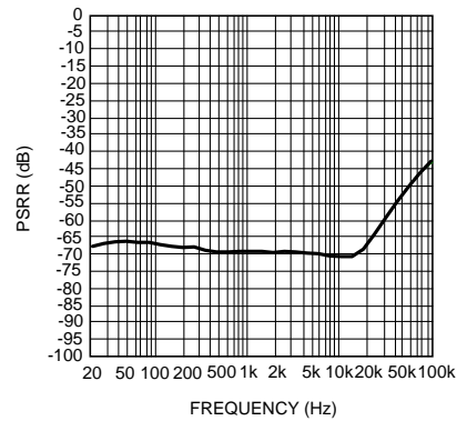
Power Supply Rejection Ratio V_{DD} = 1.5V, V_{RIPPLE} = 200mV_{PP} R_L = 16\Omega, \text{Single Ended Output} Input Terminated into 10\Omega
