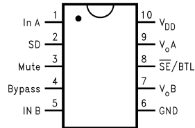
Figure 2. Top View Order Number LM4916MM See NS Package Number MUB10A for MSOP
