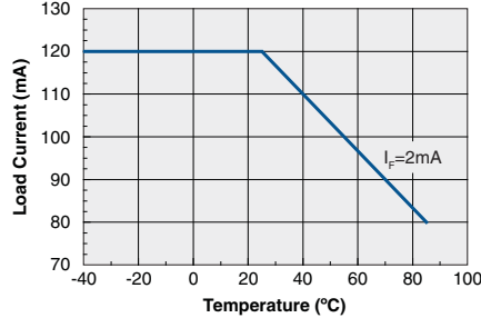
CPC1225N Typical Load Current vs. Temperature ( I_F=2\text{mA} )
