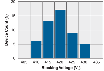
CPC1225N Typical Blocking Voltage Distribution ( T_A=25^\circ\text{C} )
