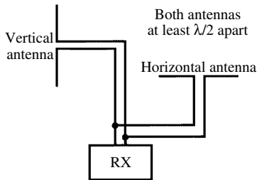
polarization diversity
