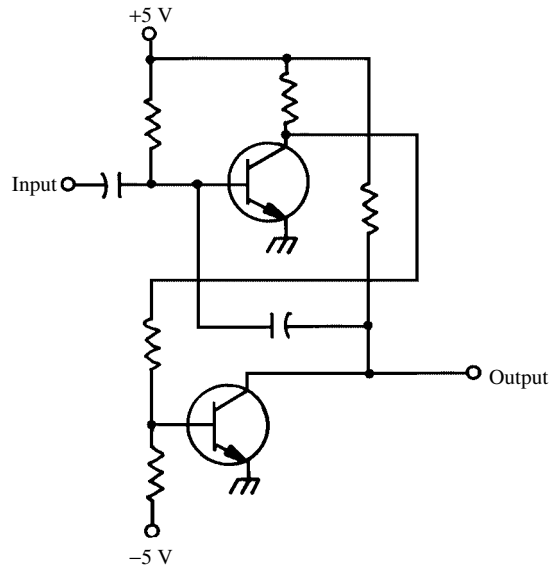
monostable multivibrator
