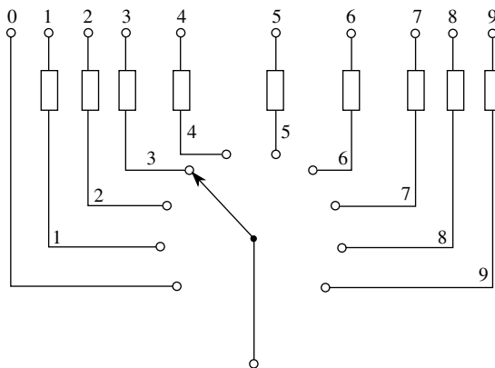
decade box
