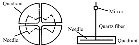
quadrant electrometer
