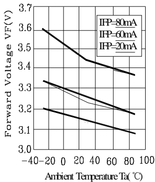
Fig.7 Ambient Temperature vs. Forward Voltage
