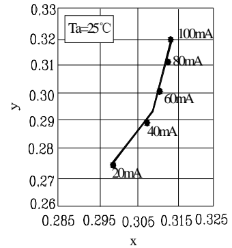
Fig.9 Forward Current vs. Chromaticity Coordinate
