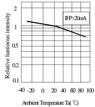
Fig.6 Luminous Intensity vs. Ambient Temperature
