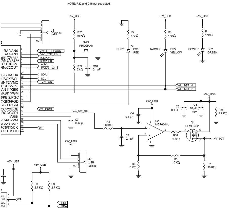
RE B-1: PICKIT™ 2 SCHEMATIC DIAGRAM (PAGE 1 OF 2)
