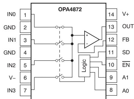
SO-14 Top View
