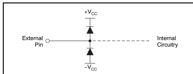
Figure 36. Internal ESD Protection
