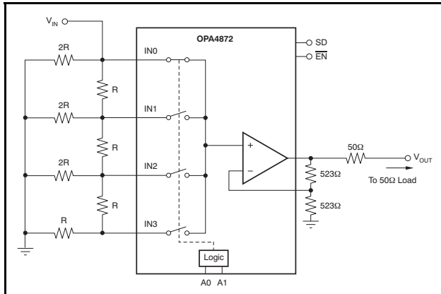
Figure 29. 2-Bit, High-Speed Attenuator, 500MHz Channel Bandwidth
