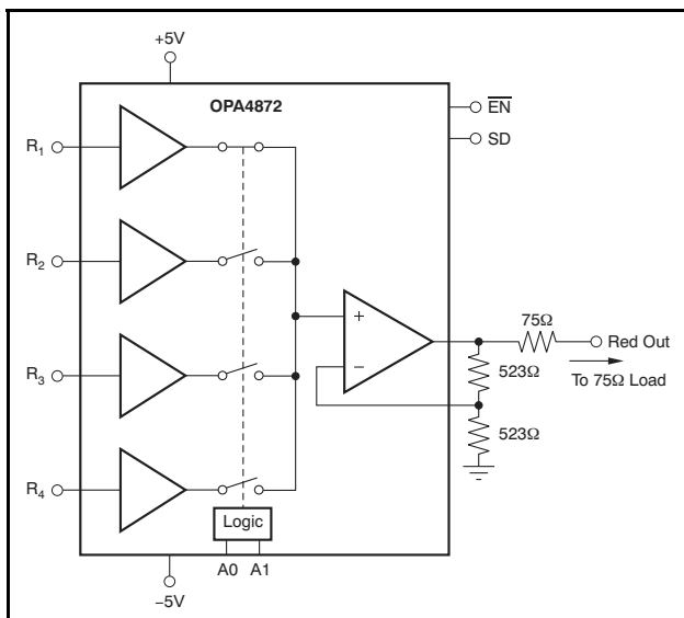
Figure 30. 4-Input RGB Router (Red Channel Shown)
