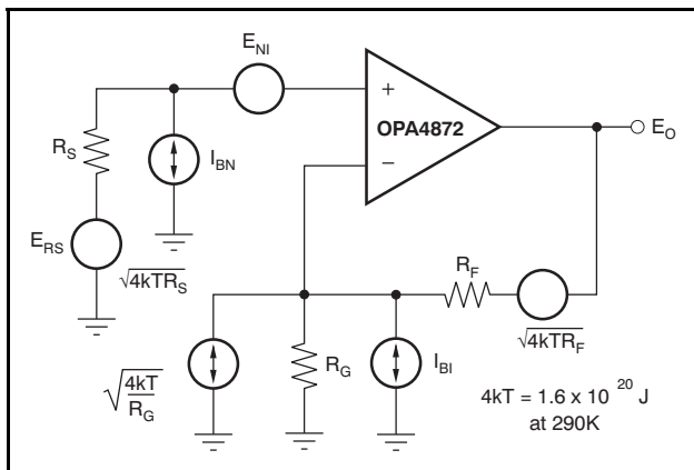
Figure 34. Op Amp Noise Analysis Model
