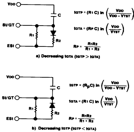
Figure 5. Guard Time Adjustment
