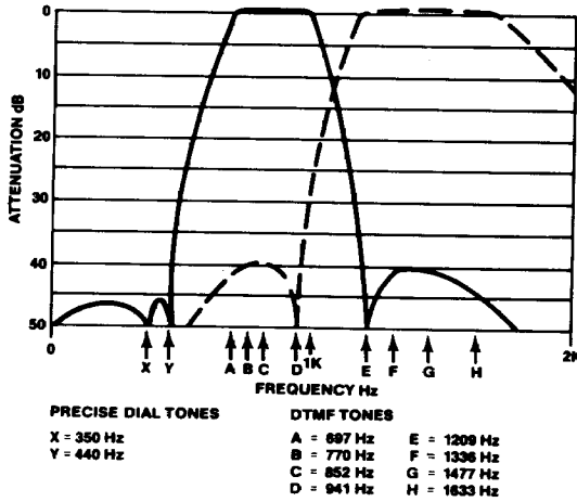
Figure 3. Typical Filter Characteristic
