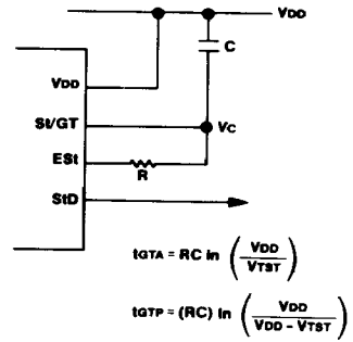
Figure 4. Basic Steering Circuit
