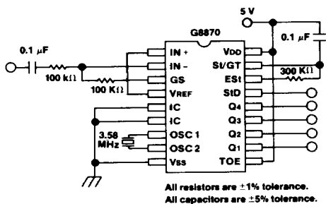
Figure 1. Single Ended Input Configuration
