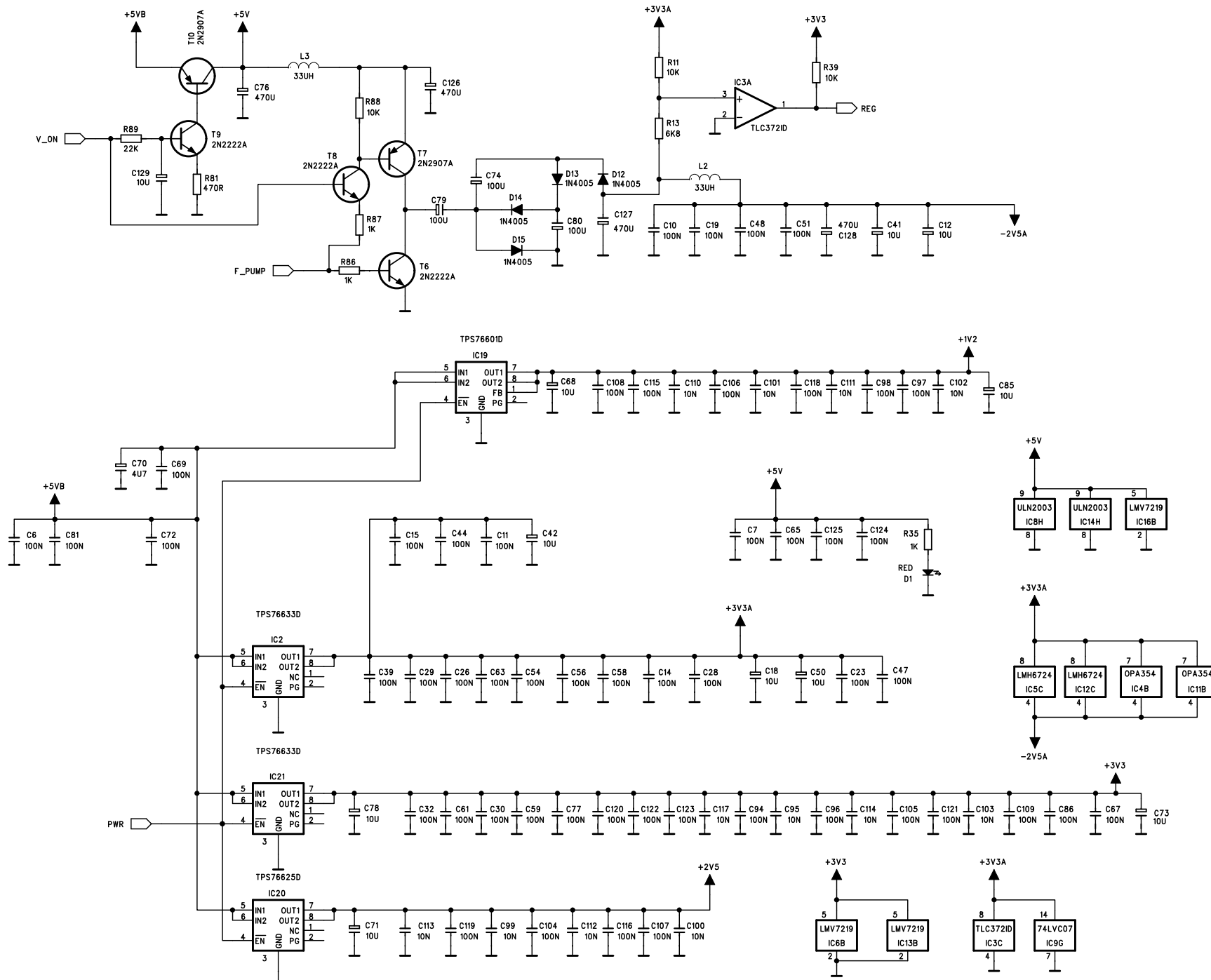
PCSU1000 POWER SUPPLY SECTION
