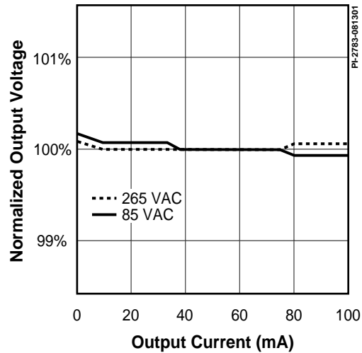
Figure 4. Load regulation at 85 VAC and 265 VAC.
